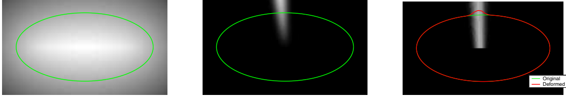
Figure 1: Simple example of the distance transform parameterization. The images show an example outline and its signed distance transform \mathbf{x} (left); an example of a displacement vector d\mathbf{x} (middle); the outline obtained by deforming the original boundary by the estimated deformation vector d\mathbf{s} and the corresponding change in the distance transform d\mathbf{x}^o (right).
